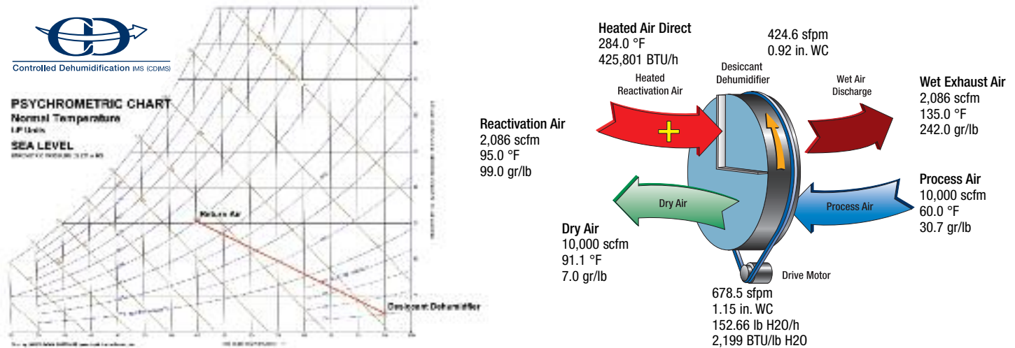
Chart 2 - Comparison of Desiccant Dehumidifier Capacity 2 60° Fahrenheit @ 40% Relative Humidity-Unoccupied
