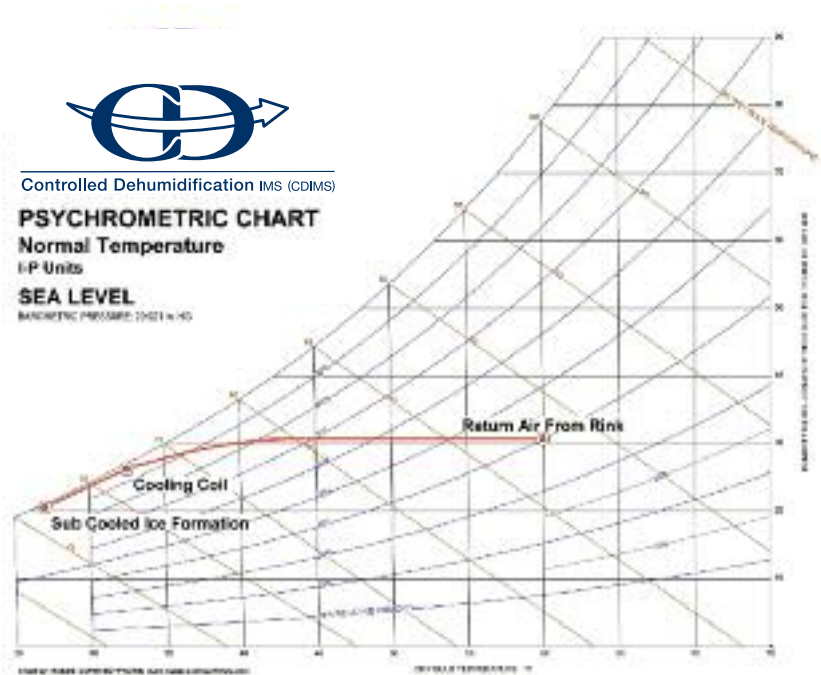
Chart 1 - Refrigeration Capacity 60° Fahrenheit @ 40% Relative Humidity-Unoccupied Typical Cold-Coil Performance
